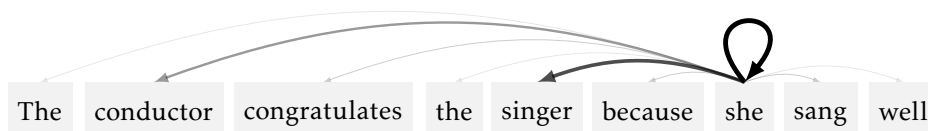
(a) Text self-attention visualization. Arrows represent self-attention weights between each token (here, a full word) and the token <she>.
