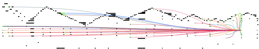
(b) Musical self-attention visualization through a piano roll representation. The tokenization in use is MIDI-like. Reproduced from (Huang et al., 2018).
