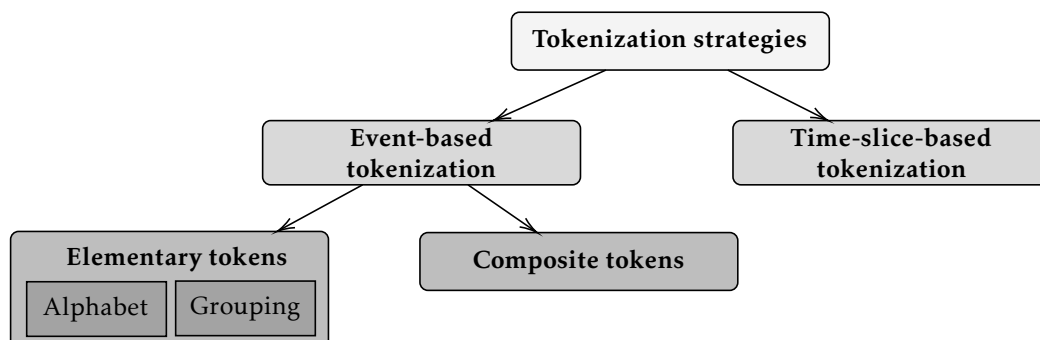
Figure 4.1: Taxonomy of tokenizations for symbolic music. Tokens are either based on regular time-slices or events. Among event-based tokenization strategies, tokens encode various features of these events: composite (or multidimensional) tokens encapsulate all these features in a single token, in contrast with elementary tokens where each musical feature is processed one after the other.
