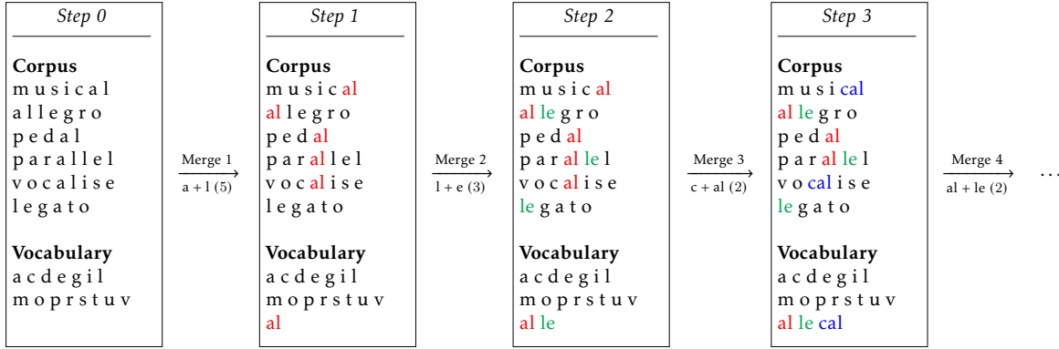
Figure 4.6: Byte-Pair Encoding (BPE) algorithm on text data. The process starts with a vocabulary composed of all characters occurring in the corpus considered as initial tokens. At step 1, the most occurring pair of tokens is ( \langle a \rangle , \langle l \rangle ) which occurs 5 times: they are merged and \langle al \rangle is added to the vocabulary. At step 2, a new token \langle le \rangle is added to the vocabulary. At step 3, a single character can be merged with an already created token ( \langle c \rangle , \langle al \rangle ) creating a new token \langle cal \rangle in the vocabulary. The algorithm then continues for a number of merges.
